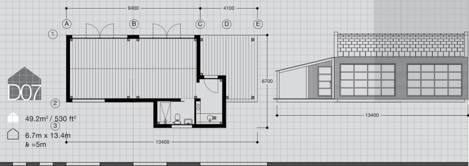
D04 49.2m 2 / 530 ft 2 6.7m x 11.2m h = 5m
