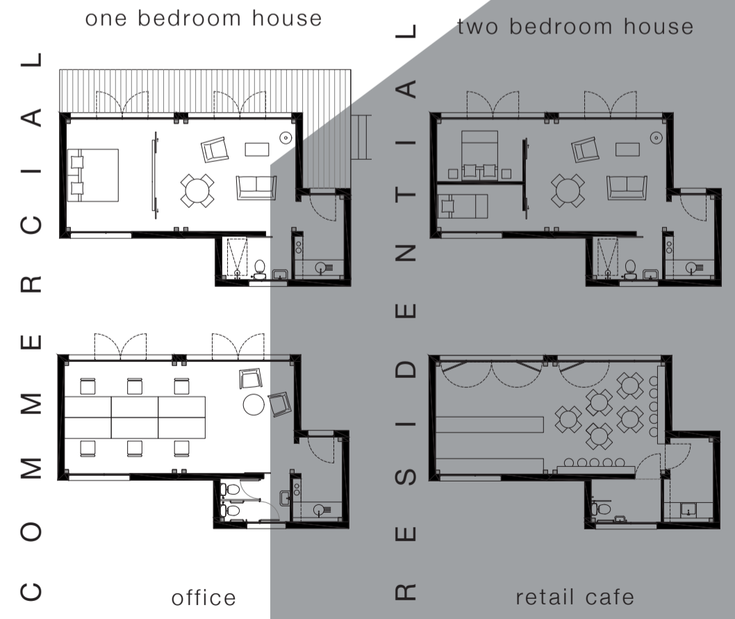
D07 49.2m 2 / 530 ft 2 6.7m x 13.4m h = 5m
