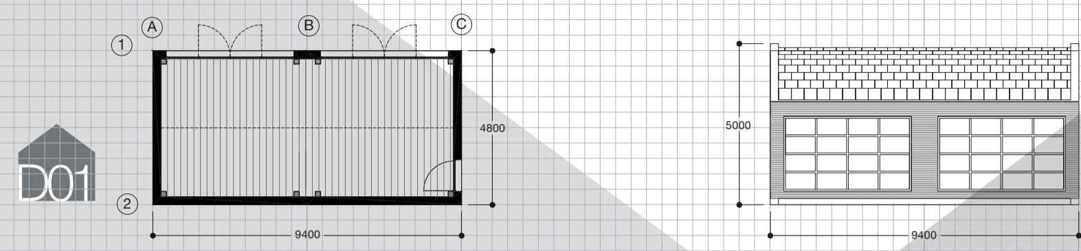
D01 40m 2 / 408 ft 2 4.8m x 9.4m h = 5m
