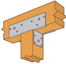
PC Beam to column connection
