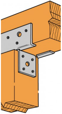
EPC Beam to column connection
